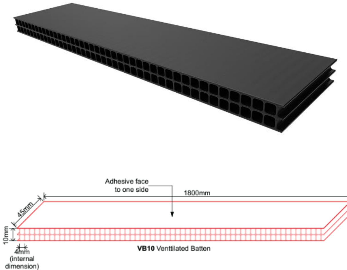
Figure 1. VENT Systems VB10 Batten nominal dimensions.
